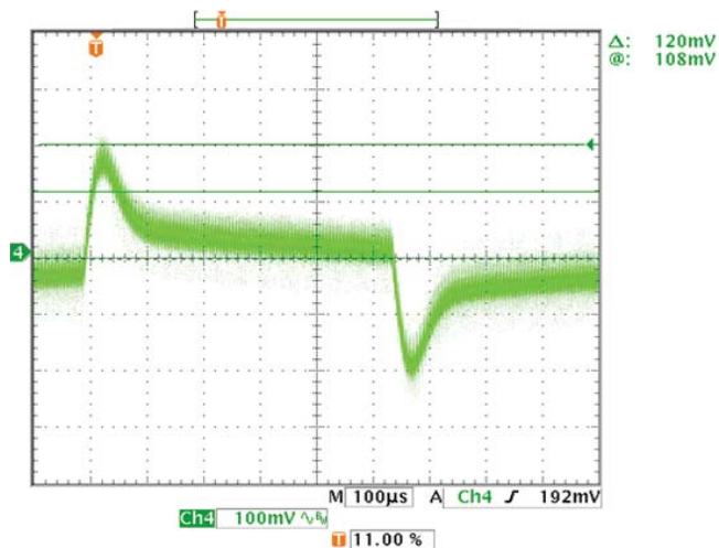
Step Load Transient Response (Vin = 48V, Vout = nom, Iout = 100 to 50% of full load 1 \mu F || 10 \mu F)
